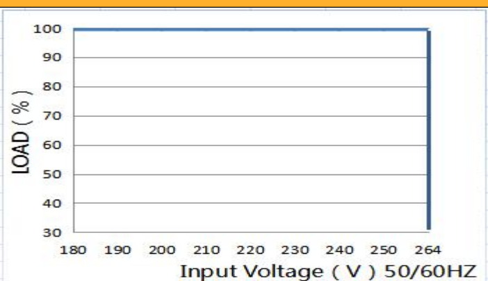
Fig. 2 Static characteristic curve
