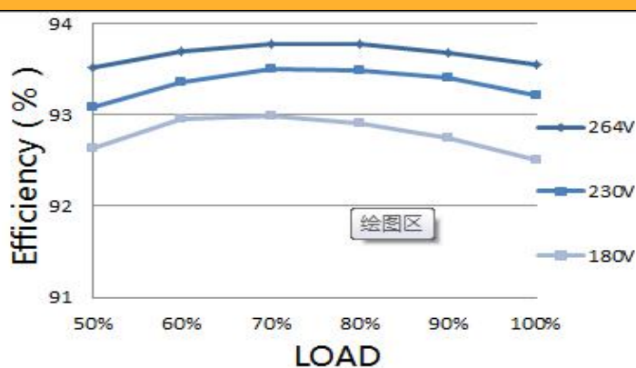
Fig.6 Efficiency-Load curve
